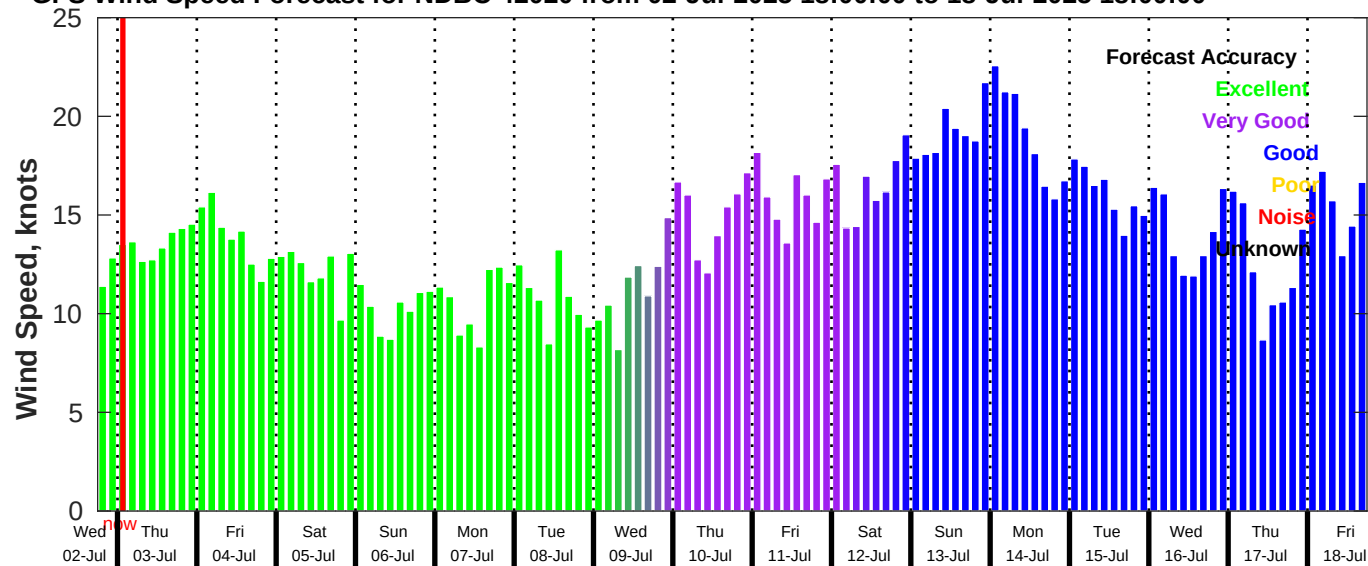
GFS Wind Speed Forecast for NDBC 42020 from 02-Jul-2025 18:00:00 to 18-Jul-2025 18:00:00
