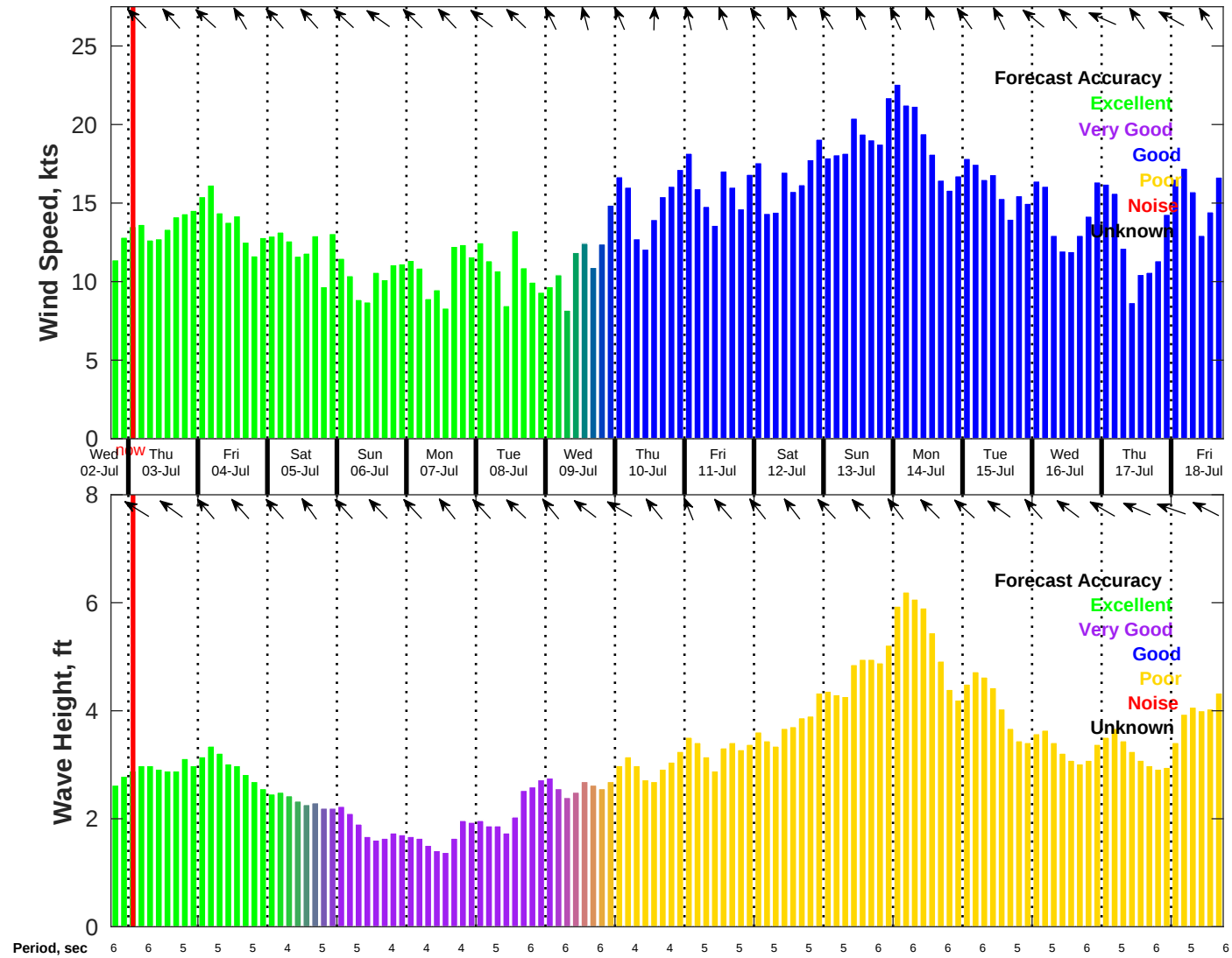
Wind & Wave Forecast for NDBC 42020 from 02-Jul-2025 18:00:00 to 18-Jul-2025 18:00:00
