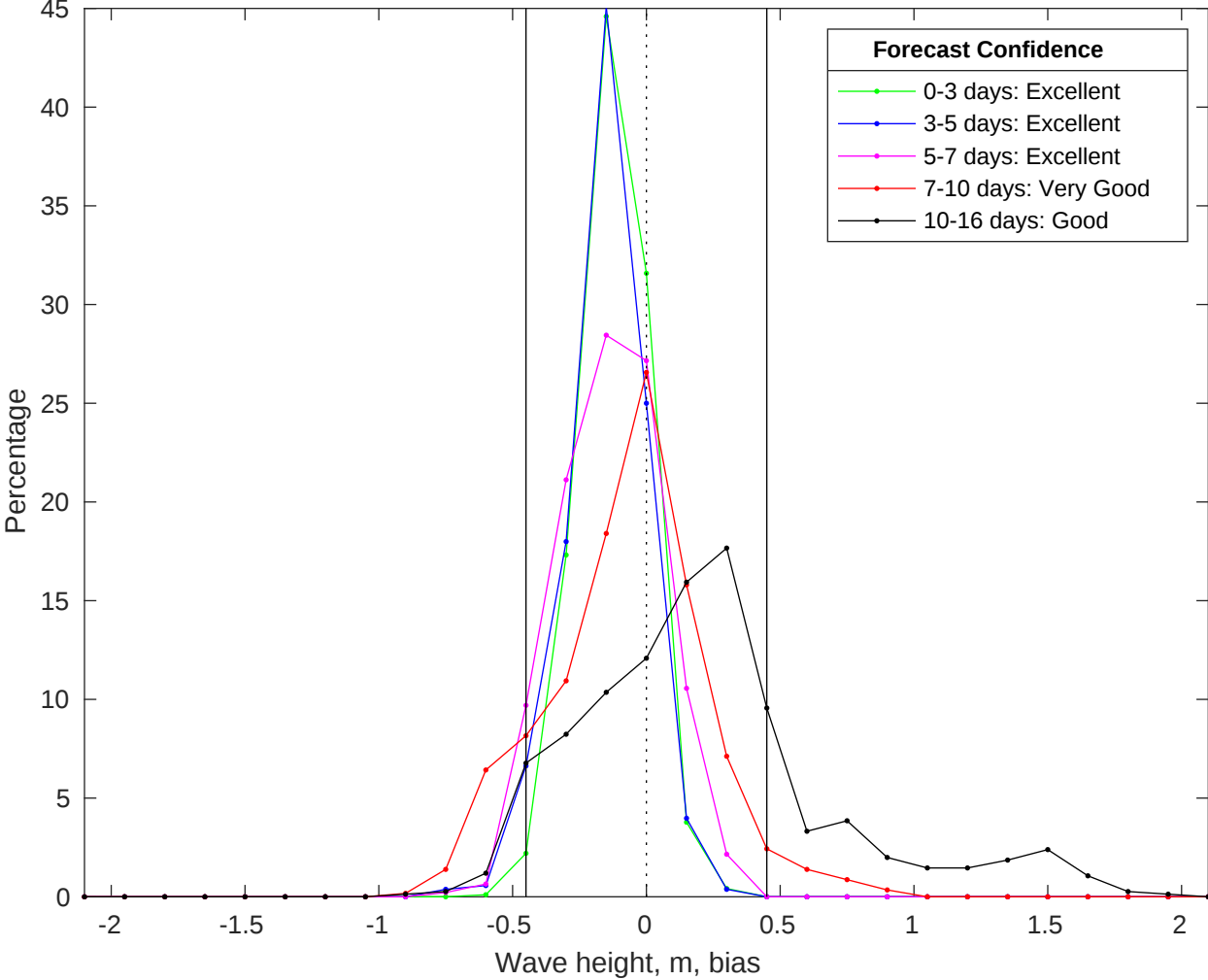
NDBC 42035 vs GFS Waves Bias Histogram: 03-Jul-2025
