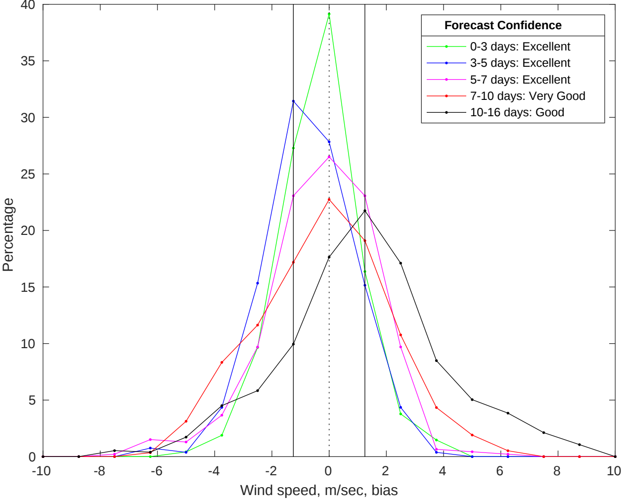
NDBC 42035 vs GFS Winds Bias Histogram: 03-Jul-2025
