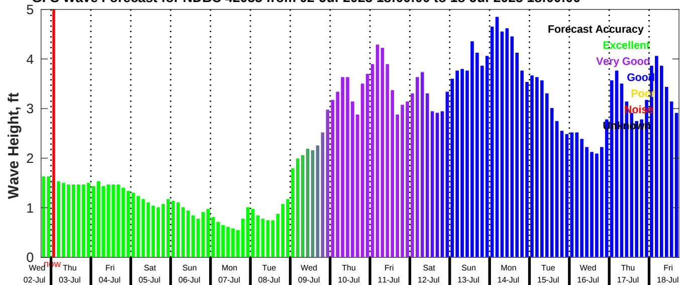
GFS Wave Forecast for NDBC 42035 from 02-Jul-2025 18:00:00 to 18-Jul-2025 18:00:00
