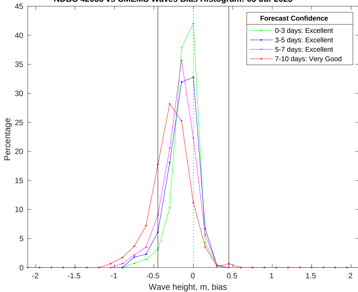
NDBC 42036 vs CMEMS Waves Bias Histogram: 03-Jul-2025
