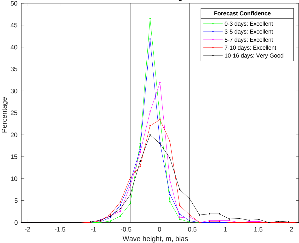
NDBC 42036 vs GFS Waves Bias Histogram: 03-Jul-2025
