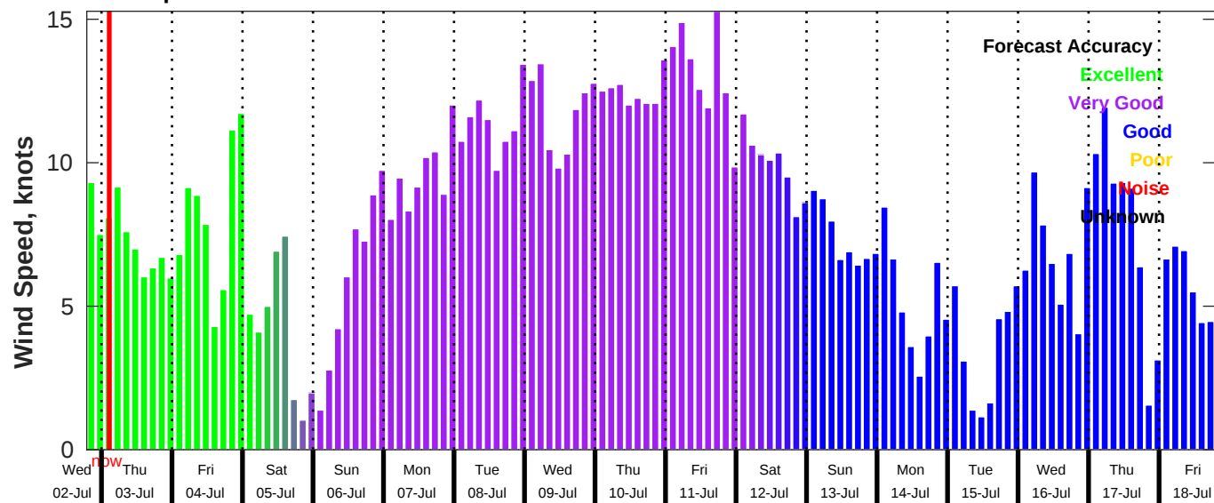
GFS Wind Speed Forecast for NDBC 42036 from 02-Jul-2025 19:00:00 to 18-Jul-2025 19:00:00
