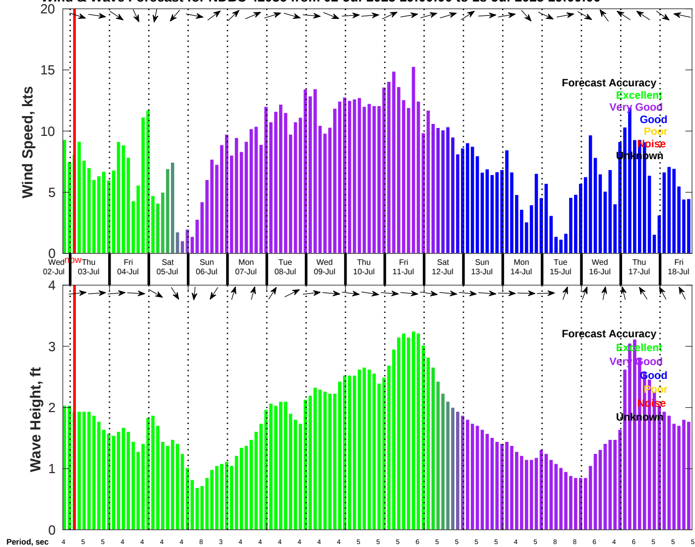
Wind & Wave Forecast for NDBC 42036 from 02-Jul-2025 19:00:00 to 18-Jul-2025 19:00:00
