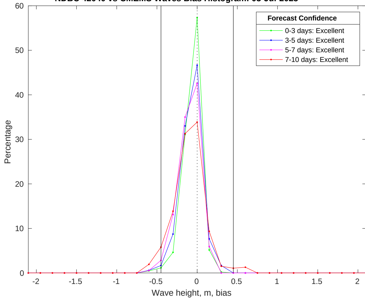
NDBC 42040 vs CMEMS Waves Bias Histogram: 03-Jul-2025
