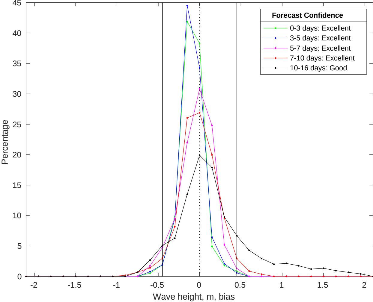
NDBC 42040 vs GFS Waves Bias Histogram: 03-Jul-2025
