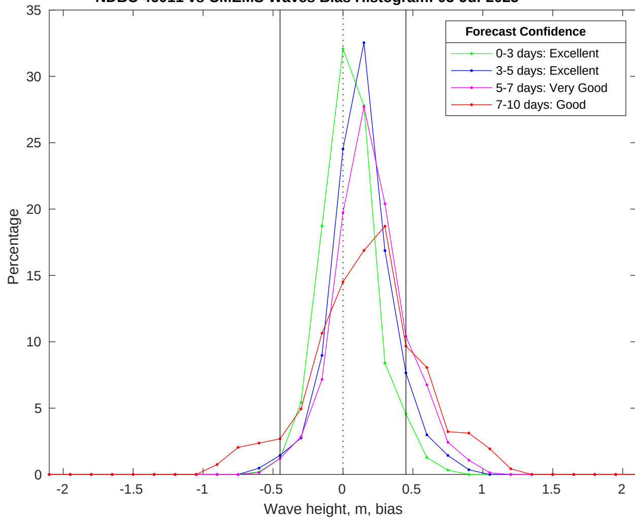
NDBC 46011 vs CMEMS Waves Bias Histogram: 03-Jul-2025
