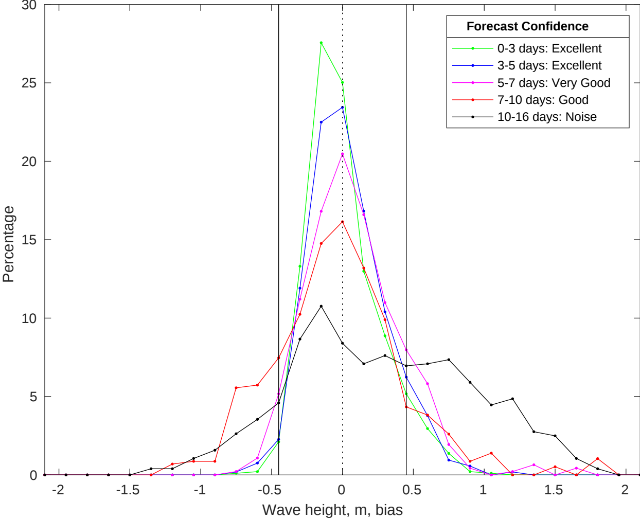
NDBC 46011 vs GFS Waves Bias Histogram: 03-Jul-2025
