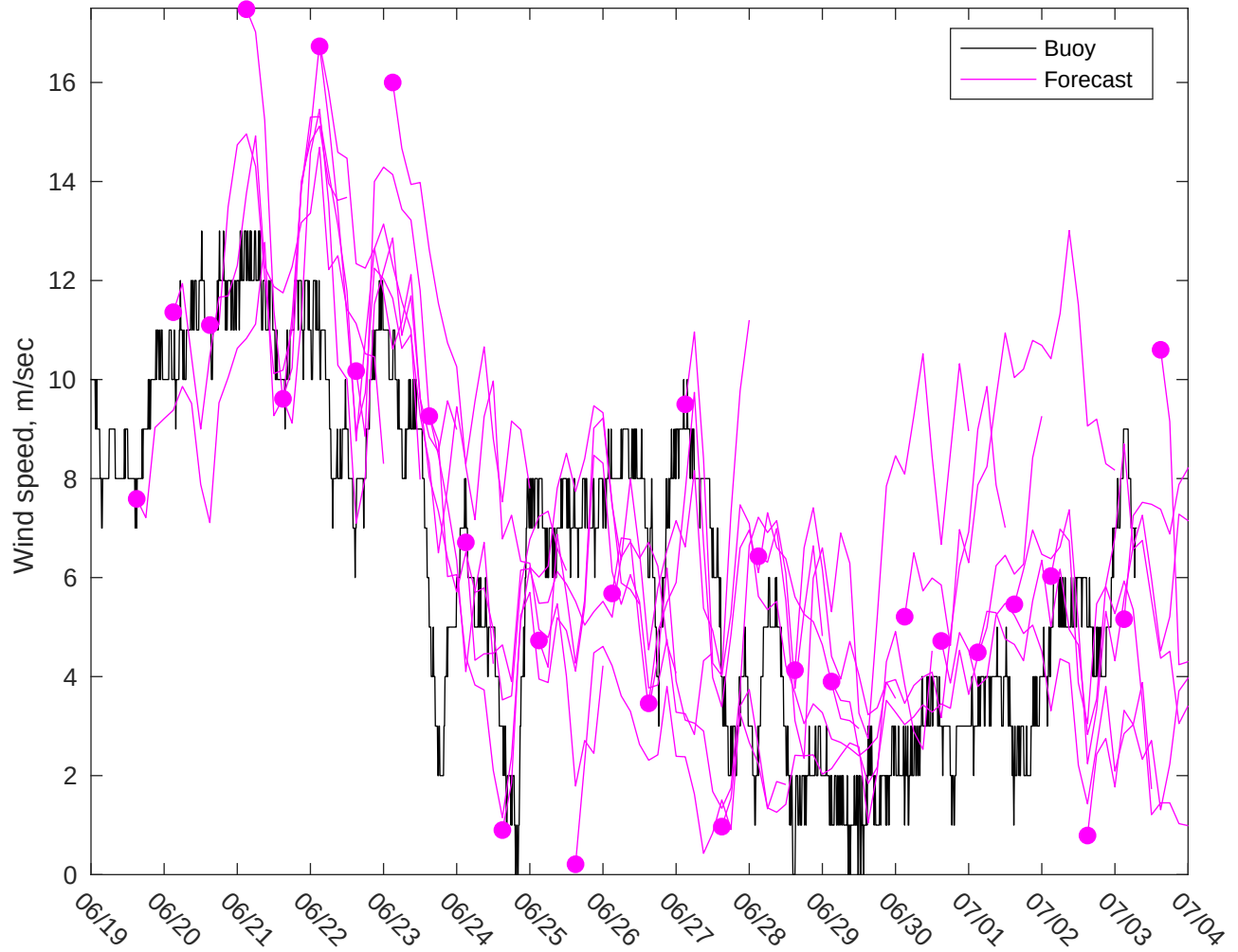
NDBC 46011 vs GFS Winds: 7 to 10 day forecast
