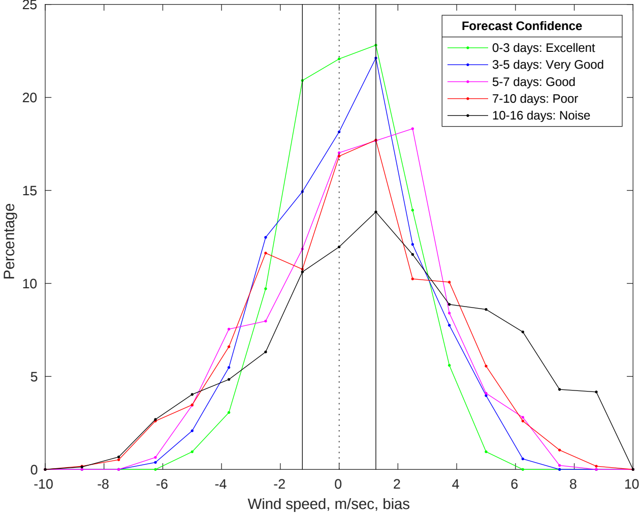
NDBC 46011 vs GFS Winds Bias Histogram: 03-Jul-2025
