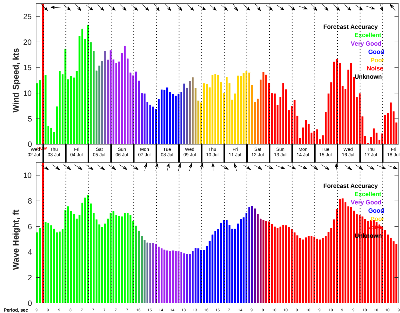
Wind & Wave Forecast for NDBC 46011 from 02-Jul-2025 16:00:00 to 18-Jul-2025 16:00:00
