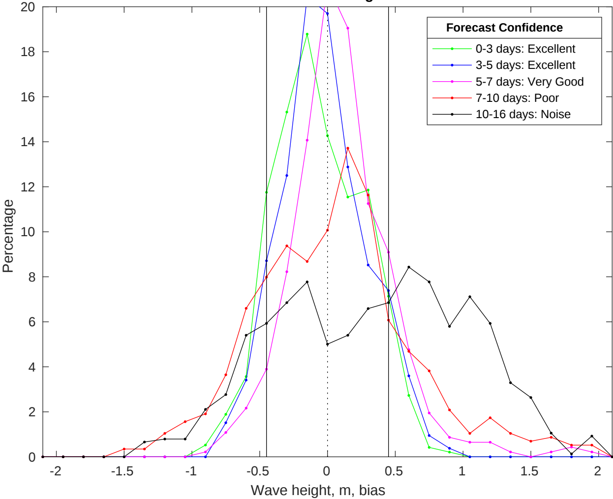
NDBC 46028 vs GFS Waves Bias Histogram: 03-Jul-2025
