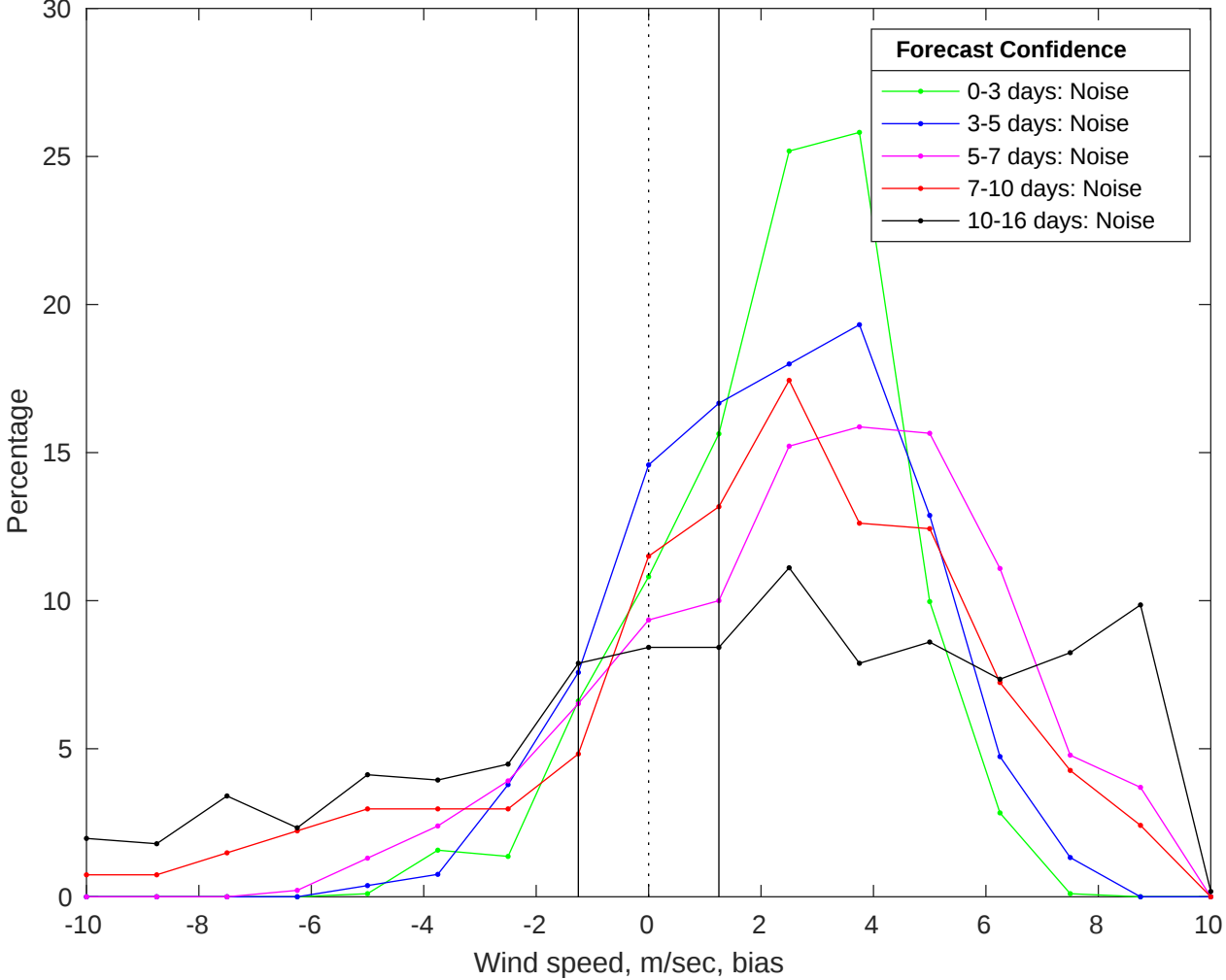
NDBC 46028 vs GFS Winds Bias Histogram: 03-Jul-2025
