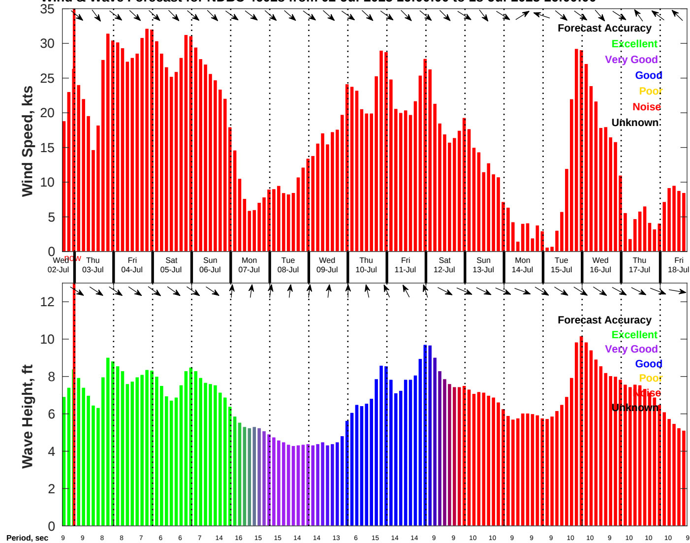
Wind & Wave Forecast for NDBC 46028 from 02-Jul-2025 16:00:00 to 18-Jul-2025 16:00:00
