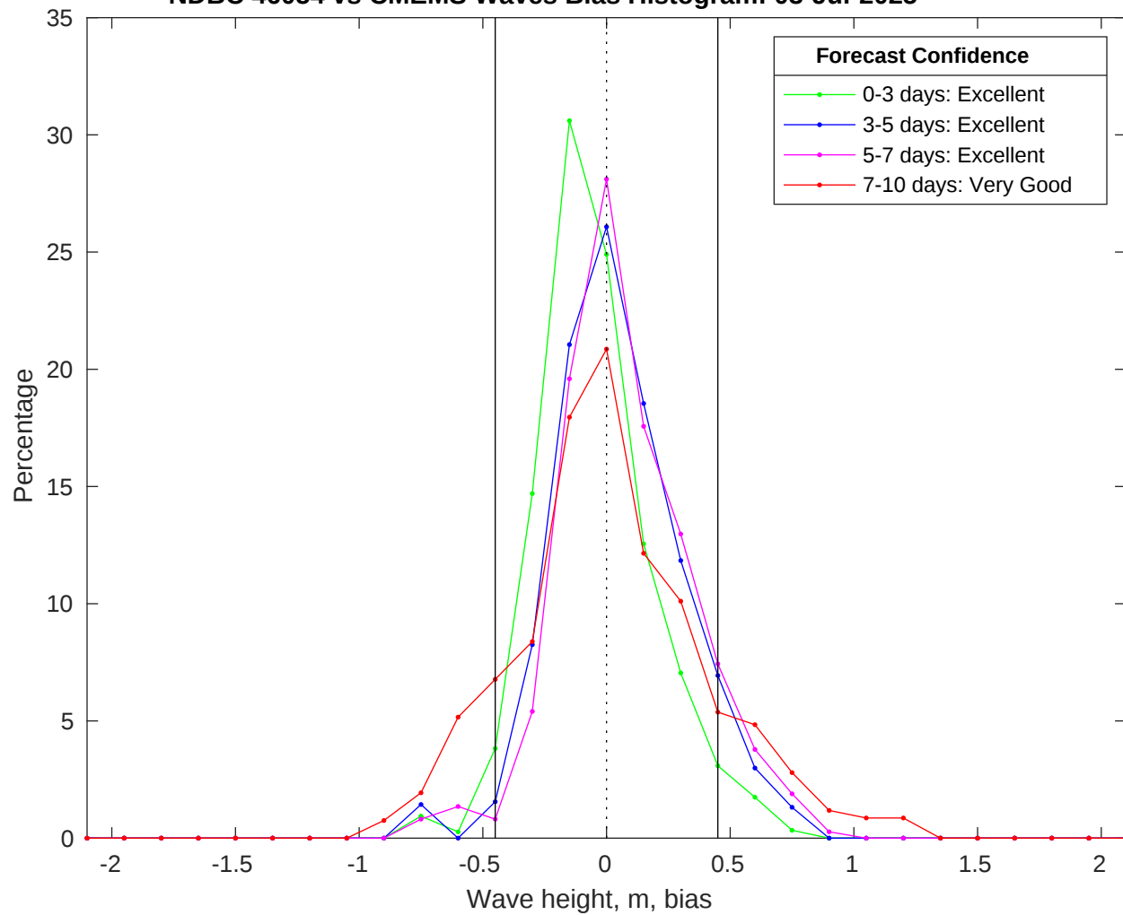
NDBC 46054 vs CMEMS Waves Bias Histogram: 03-Jul-2025
