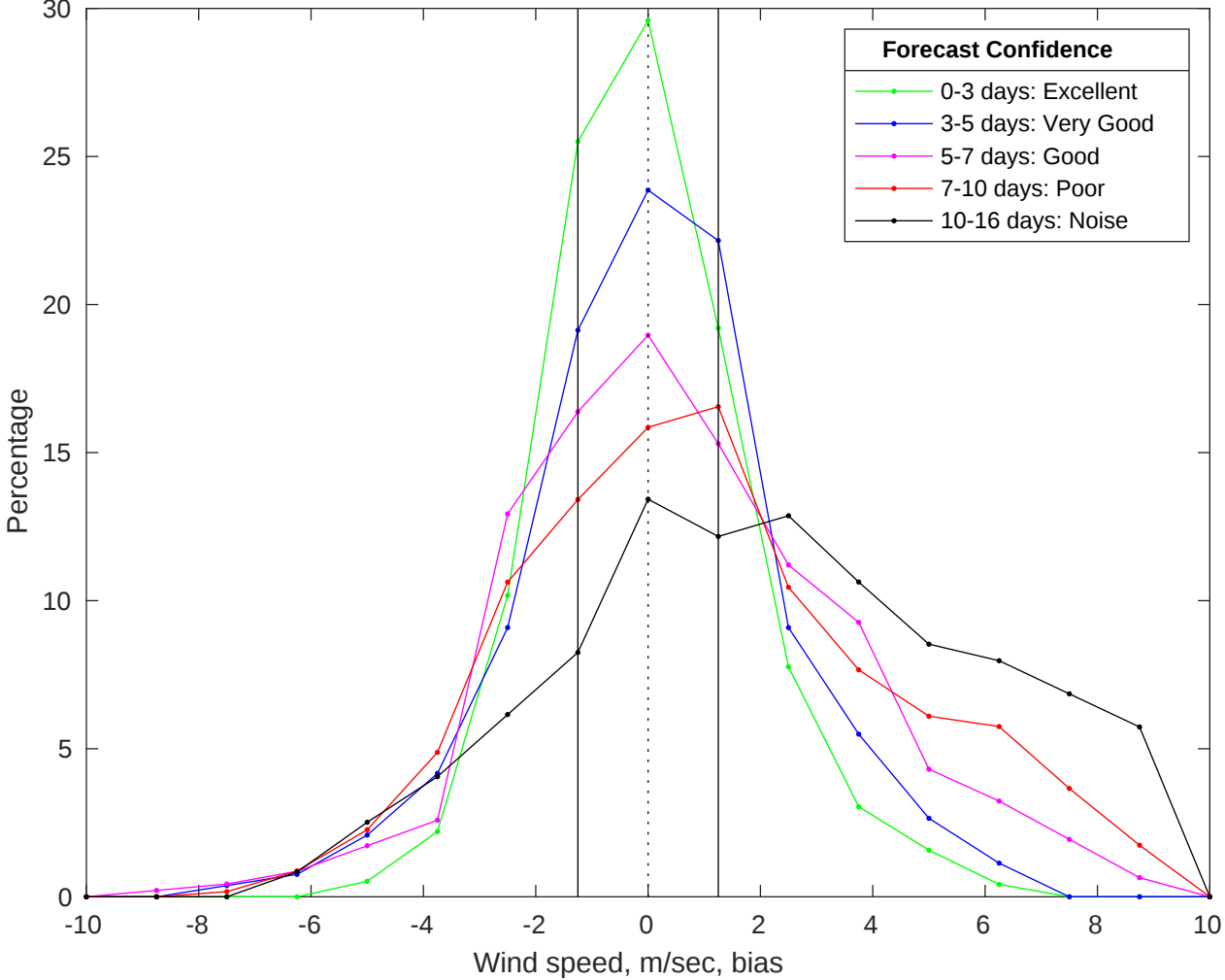
NDBC 46054 vs GFS Winds Bias Histogram: 03-Jul-2025
