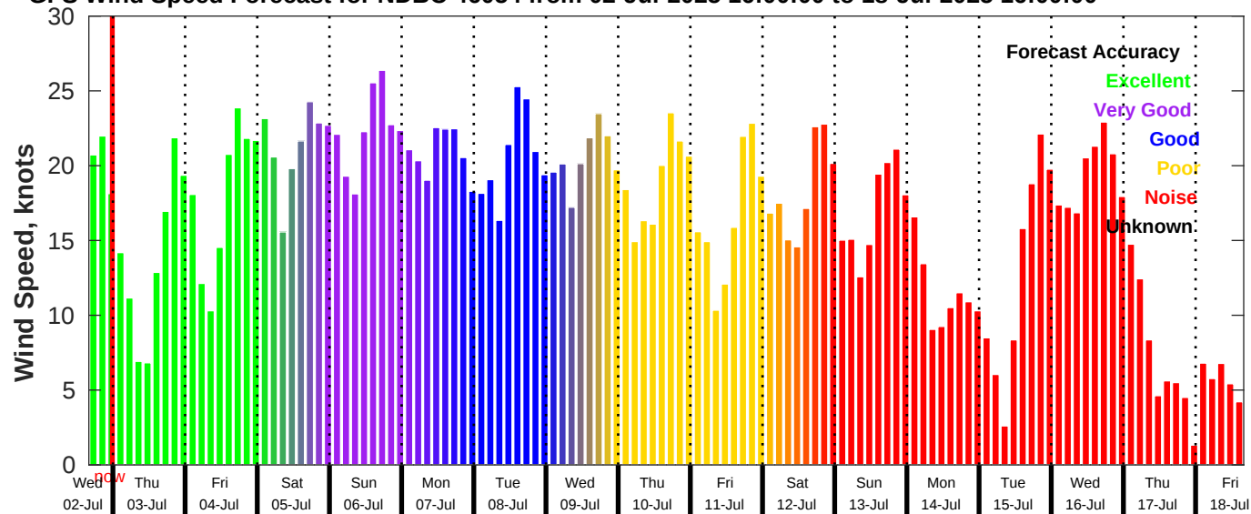
GFS Wind Speed Forecast for NDBC 46054 from 02-Jul-2025 16:00:00 to 18-Jul-2025 16:00:00
