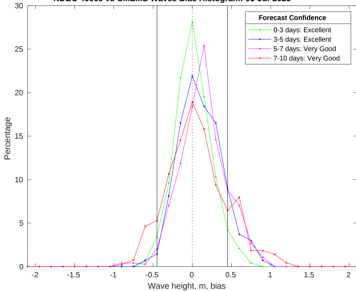
NDBC 46069 vs CMEMS Waves Bias Histogram: 03-Jul-2025
