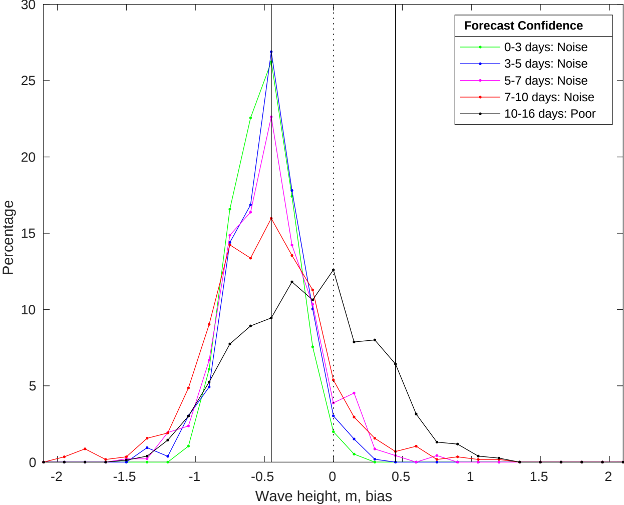
NDBC 46069 vs GFS Waves Bias Histogram: 03-Jul-2025
