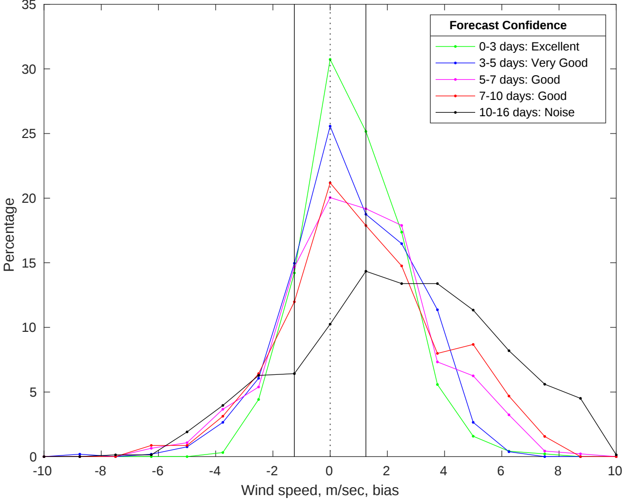
NDBC 46069 vs GFS Winds Bias Histogram: 03-Jul-2025
