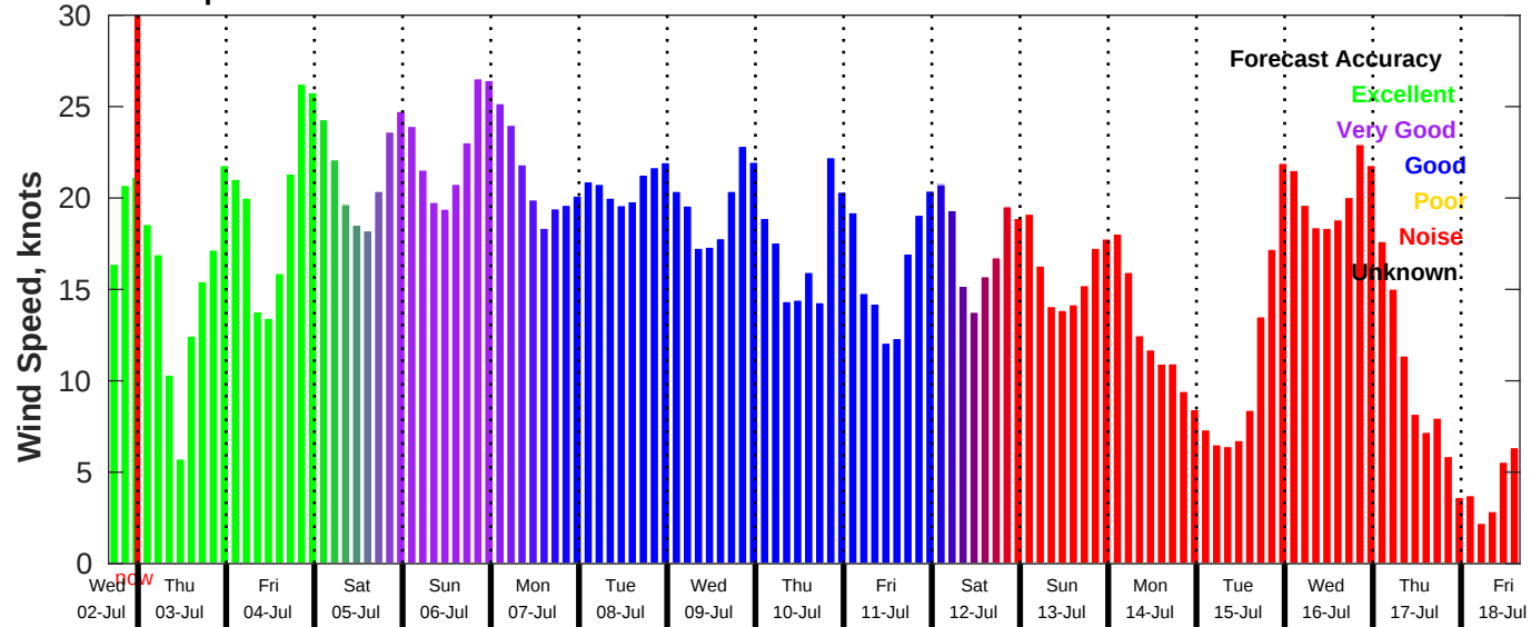
GFS Wind Speed Forecast for NDBC 46069 from 02-Jul-2025 16:00:00 to 18-Jul-2025 16:00:00
