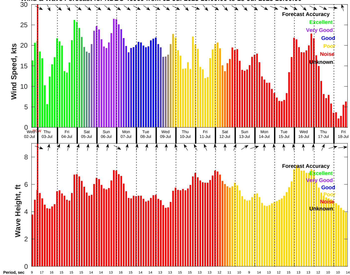
Wind & Wave Forecast for NDBC 46069 from 02-Jul-2025 16:00:00 to 18-Jul-2025 16:00:00
