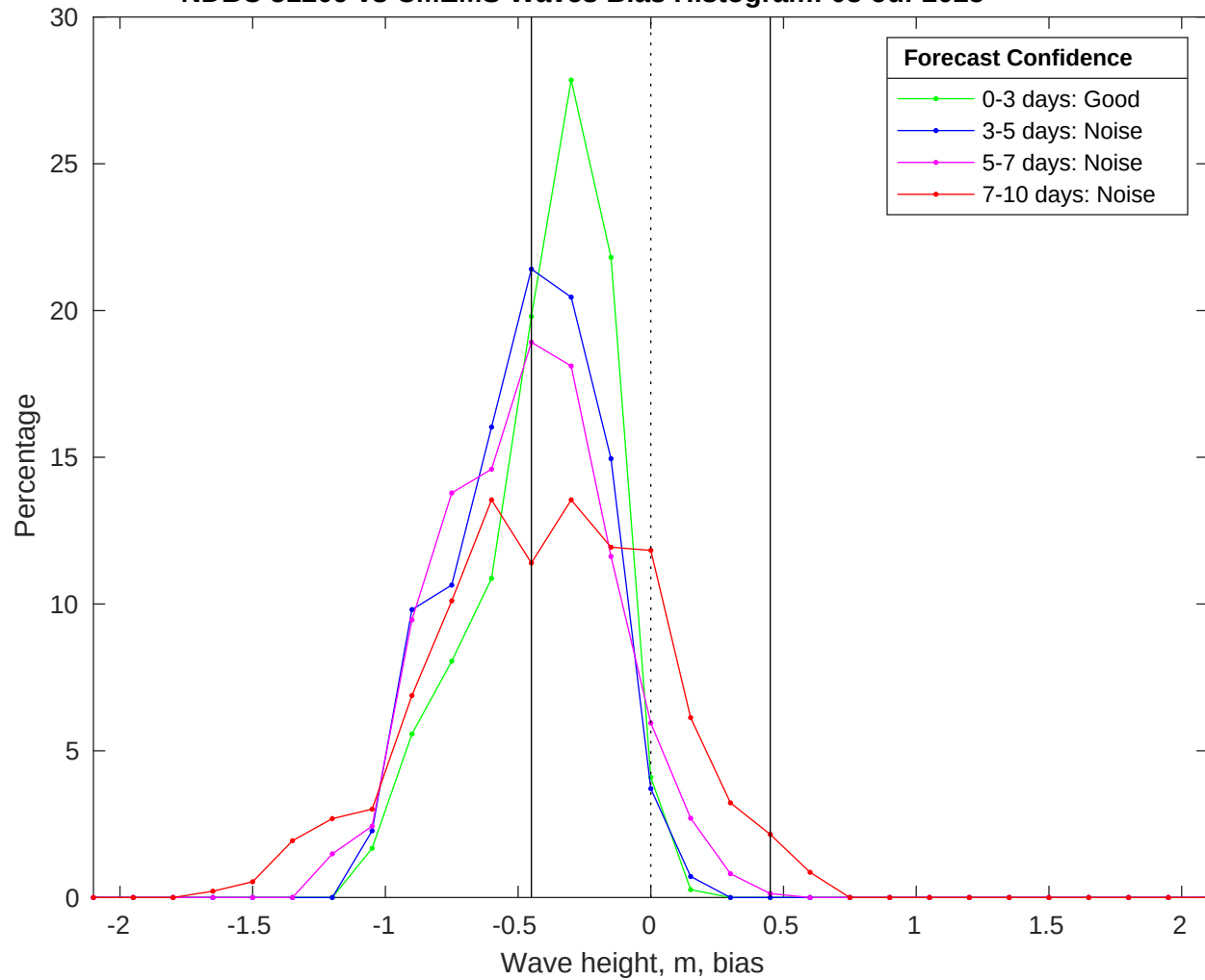
NDBC 51209 vs CMEMS Waves Bias Histogram: 03-Jul-2025
