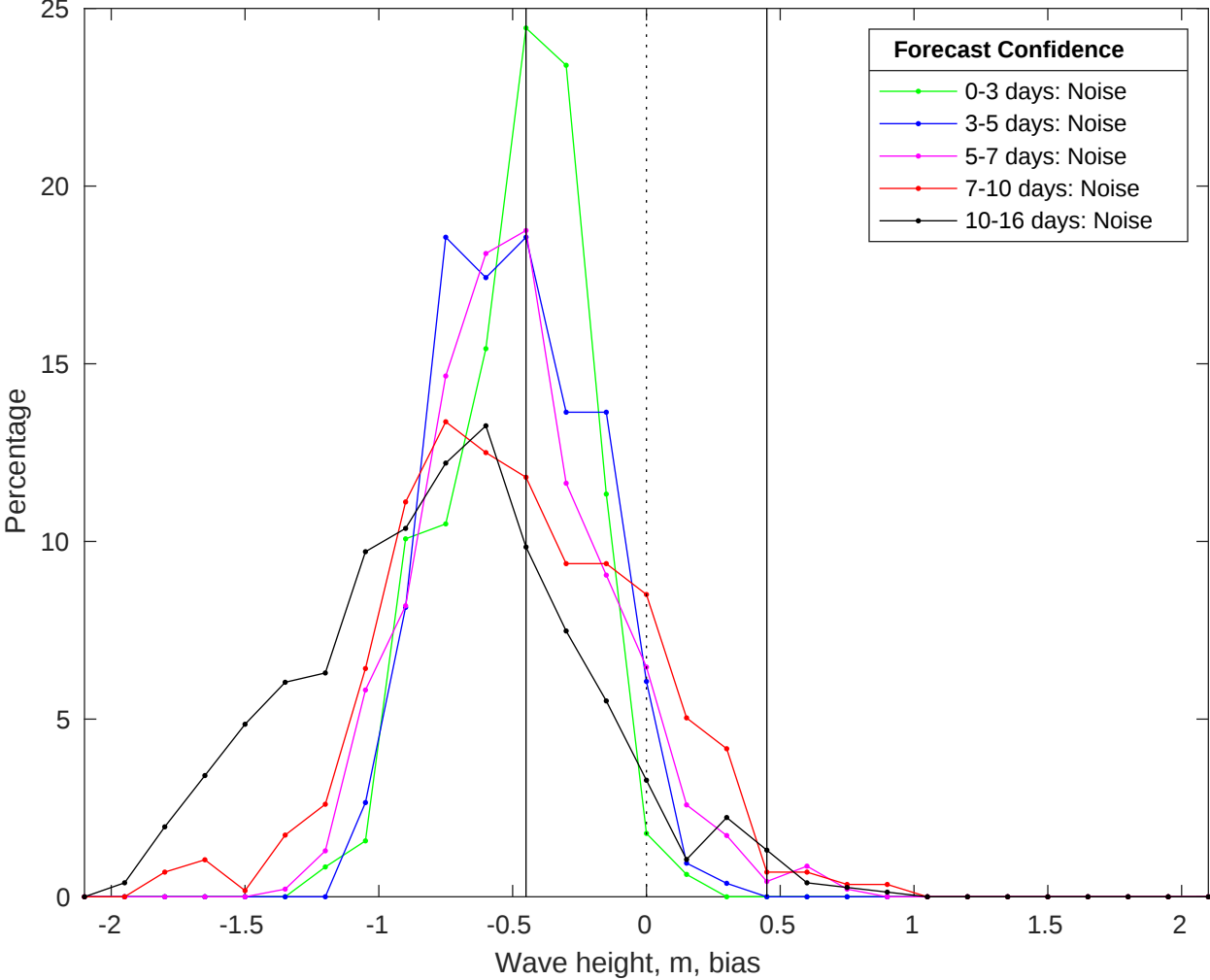
NDBC 51209 vs GFS Waves Bias Histogram: 03-Jul-2025
