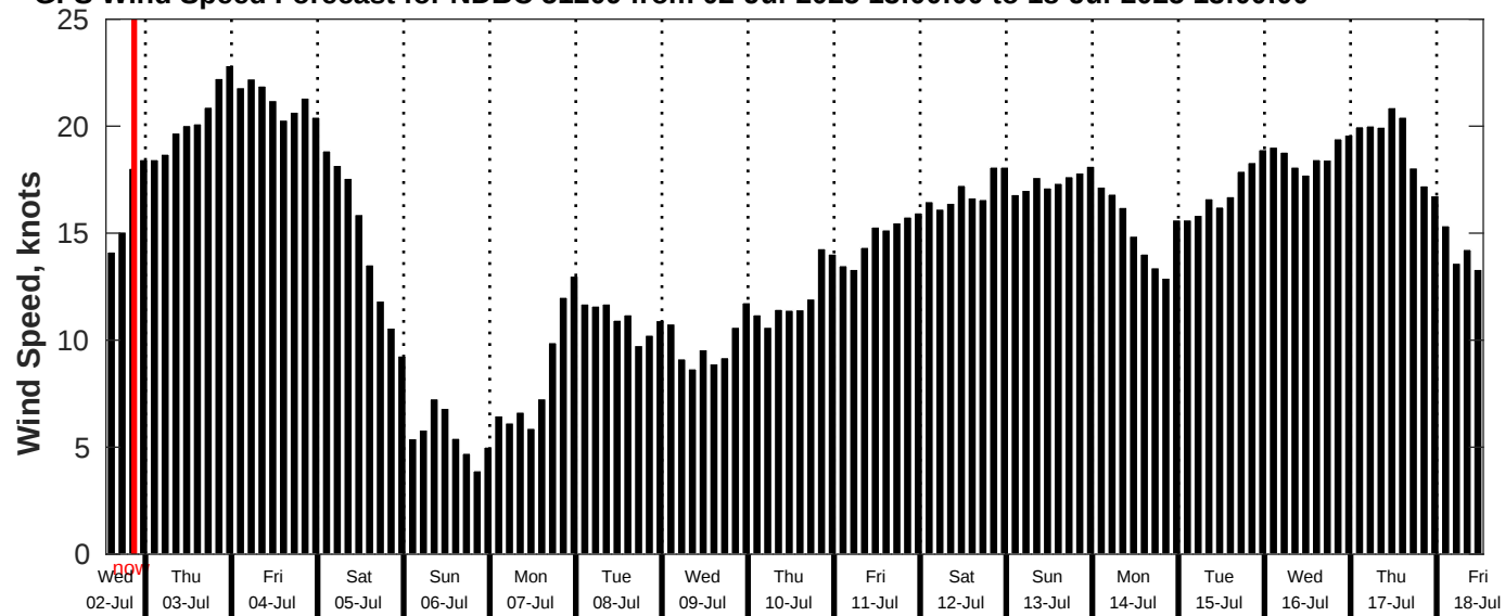
GFS Wind Speed Forecast for NDBC 51209 from 02-Jul-2025 13:00:00 to 18-Jul-2025 13:00:00
