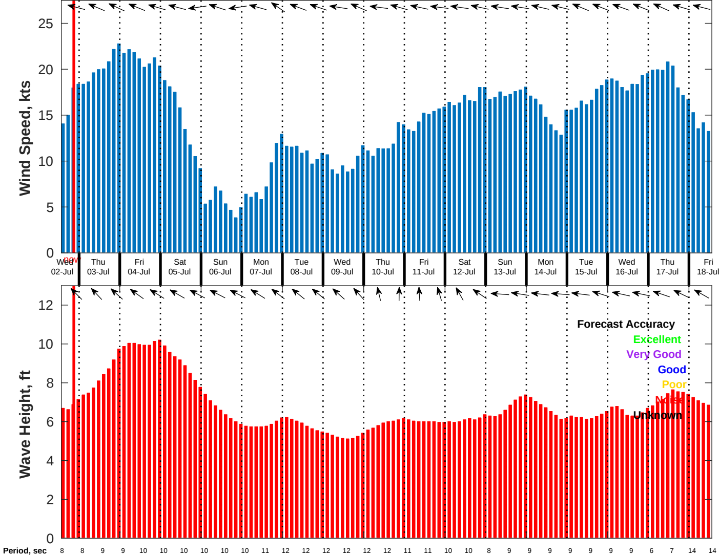
Wind & Wave Forecast for NDBC 51209 from 02-Jul-2025 13:00:00 to 18-Jul-2025 13:00:00
