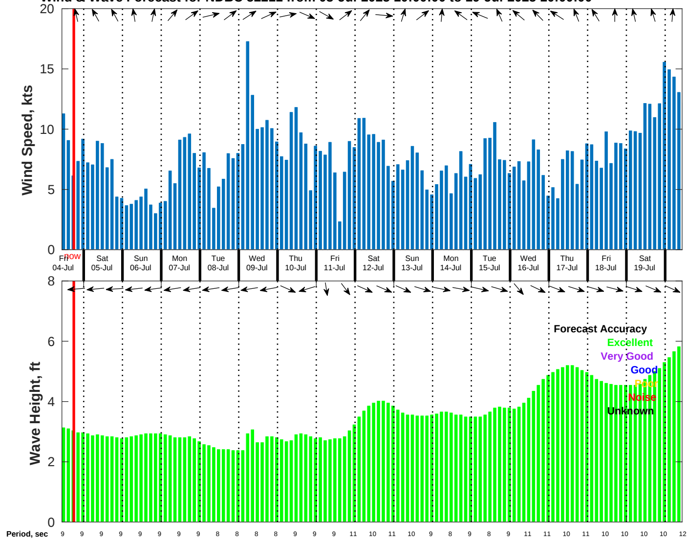
Wind & Wave Forecast for NDBC 52211 from 03-Jul-2025 10:00:00 to 19-Jul-2025 10:00:00
