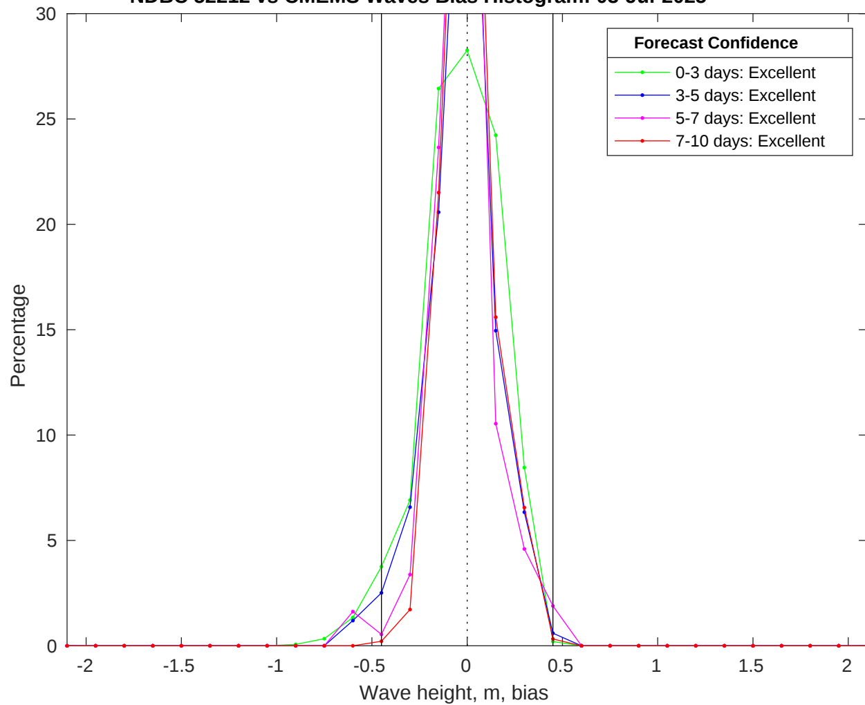
NDBC 52212 vs CMEMS Waves Bias Histogram: 03-Jul-2025
