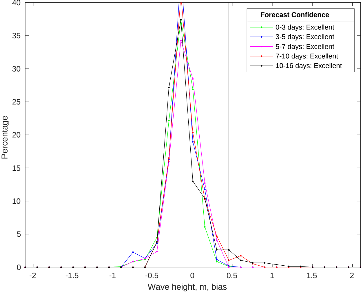
NDBC 52212 vs GFS Waves Bias Histogram: 03-Jul-2025
