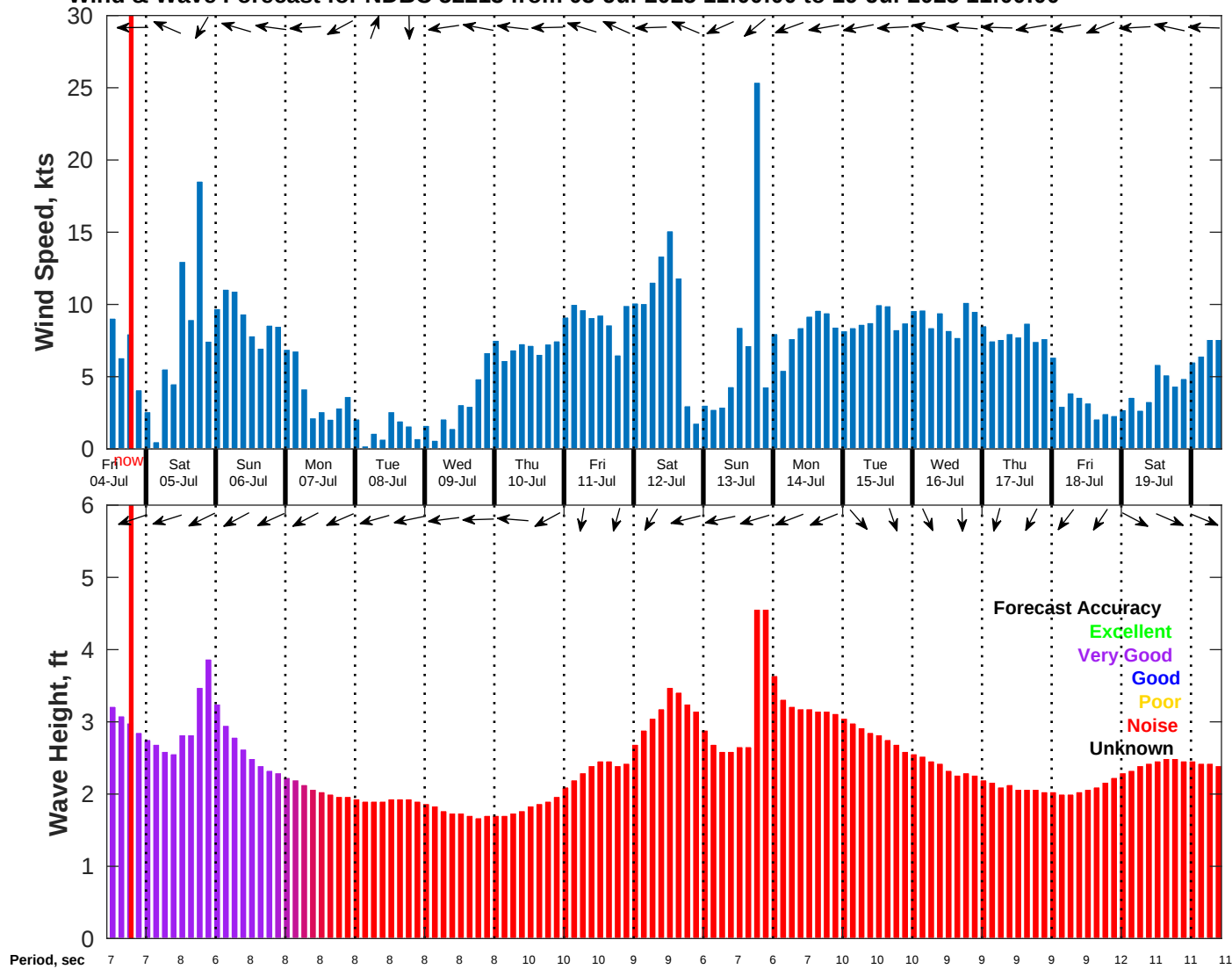
Wind & Wave Forecast for NDBC 52213 from 03-Jul-2025 11:00:00 to 19-Jul-2025 11:00:00
