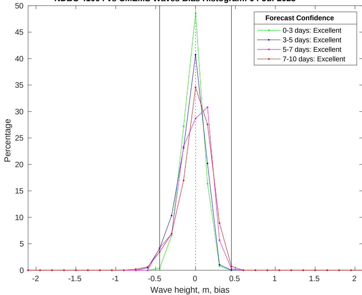
NDBC 41004 vs CMEMS Waves Bias Histogram: 04-Jul-2025
