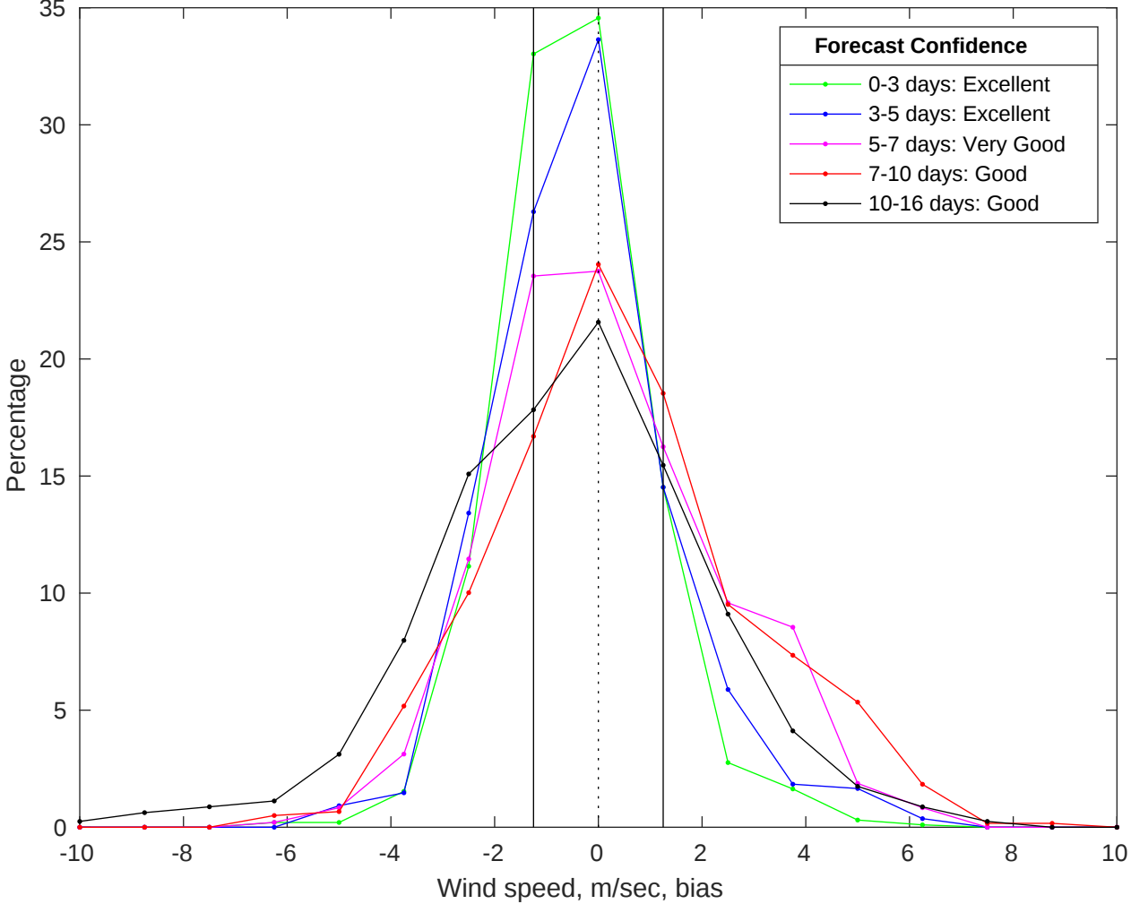
NDBC 41004 vs GFS Winds Bias Histogram: 04-Jul-2025
