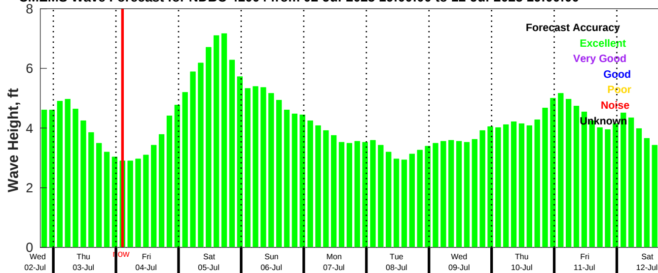
CMEMS Wave Forecast for NDBC 41004 from 02-Jul-2025 19:00:00 to 12-Jul-2025 19:00:00
