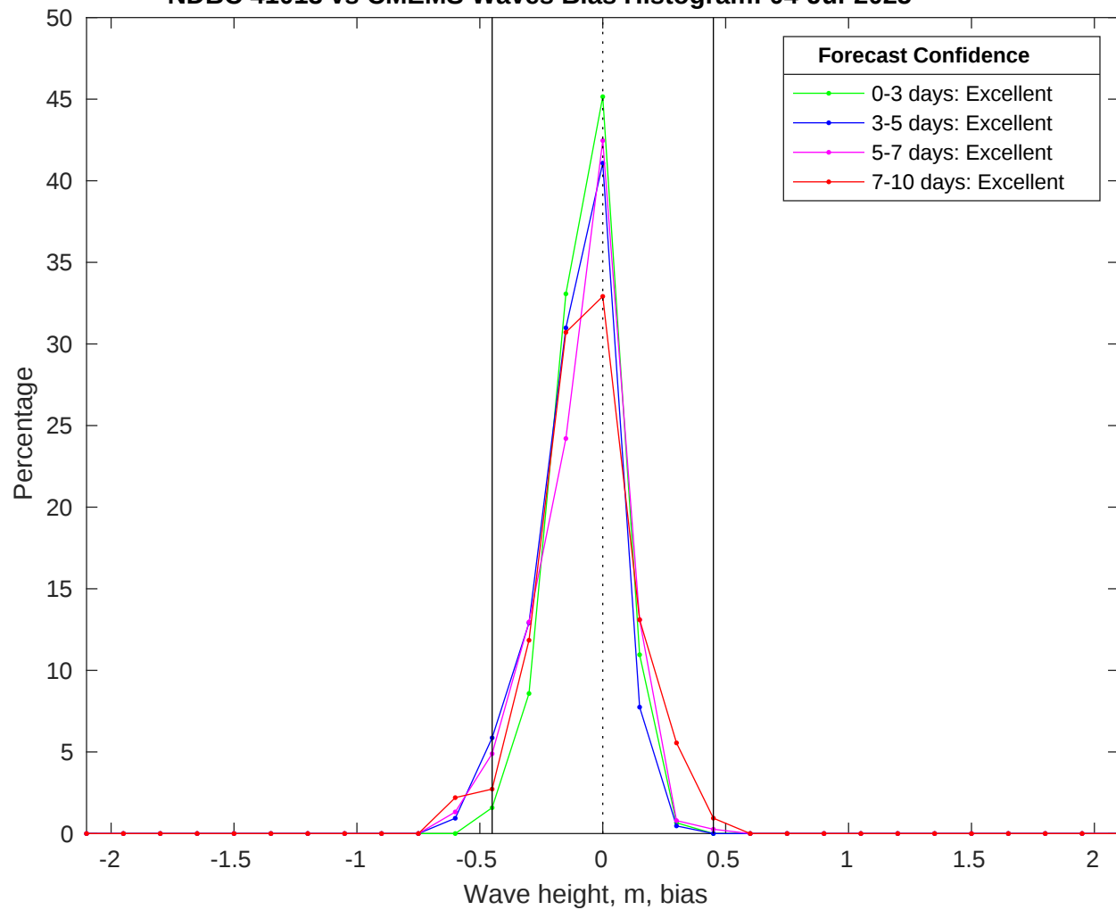
NDBC 41013 vs CMEMS Waves Bias Histogram: 04-Jul-2025
