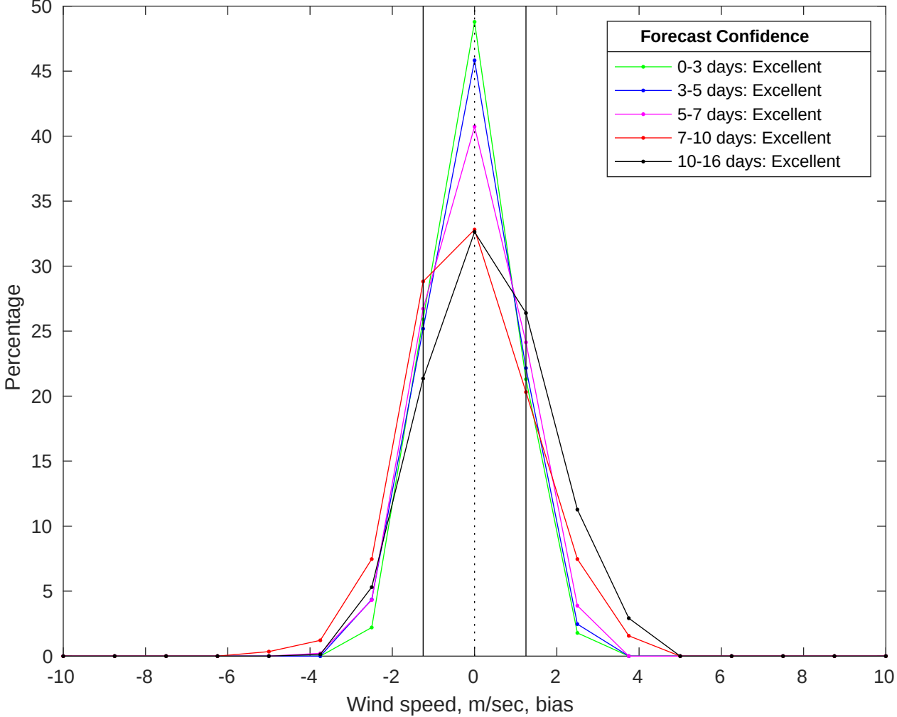
NDBC 41040 vs GFS Winds Bias Histogram: 04-Jul-2025
