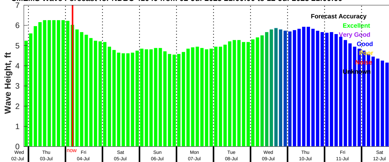
CMEMS Wave Forecast for NDBC 41040 from 02-Jul-2025 21:00:00 to 12-Jul-2025 21:00:00
