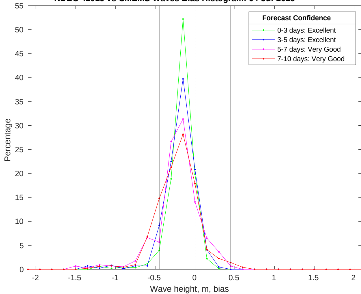
NDBC 42019 vs CMEMS Waves Bias Histogram: 04-Jul-2025
