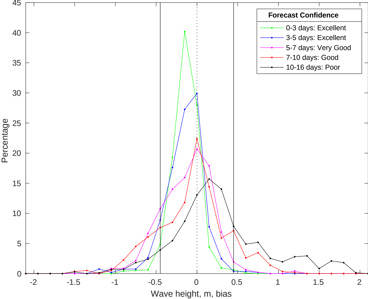
NDBC 42019 vs GFS Waves Bias Histogram: 04-Jul-2025
