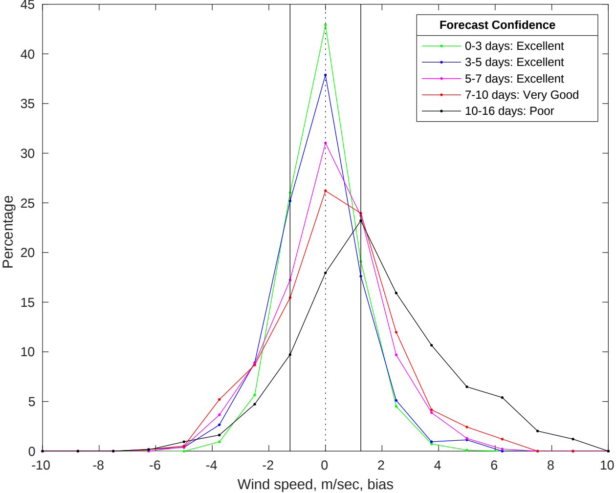
NDBC 42019 vs GFS Winds Bias Histogram: 04-Jul-2025
