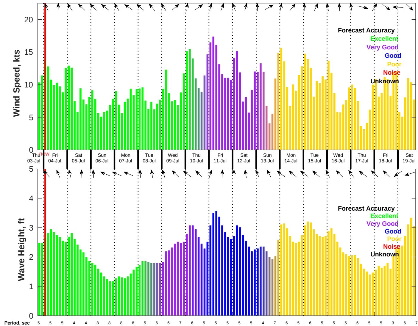
Wind & Wave Forecast for NDBC 42019 from 03-Jul-2025 18:00:00 to 19-Jul-2025 18:00:00
