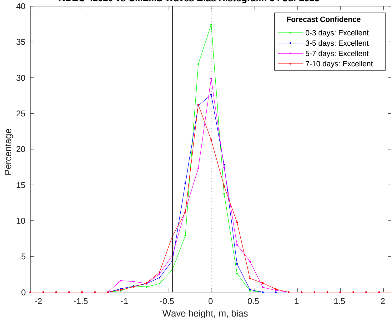
NDBC 42020 vs CMEMS Waves Bias Histogram: 04-Jul-2025
