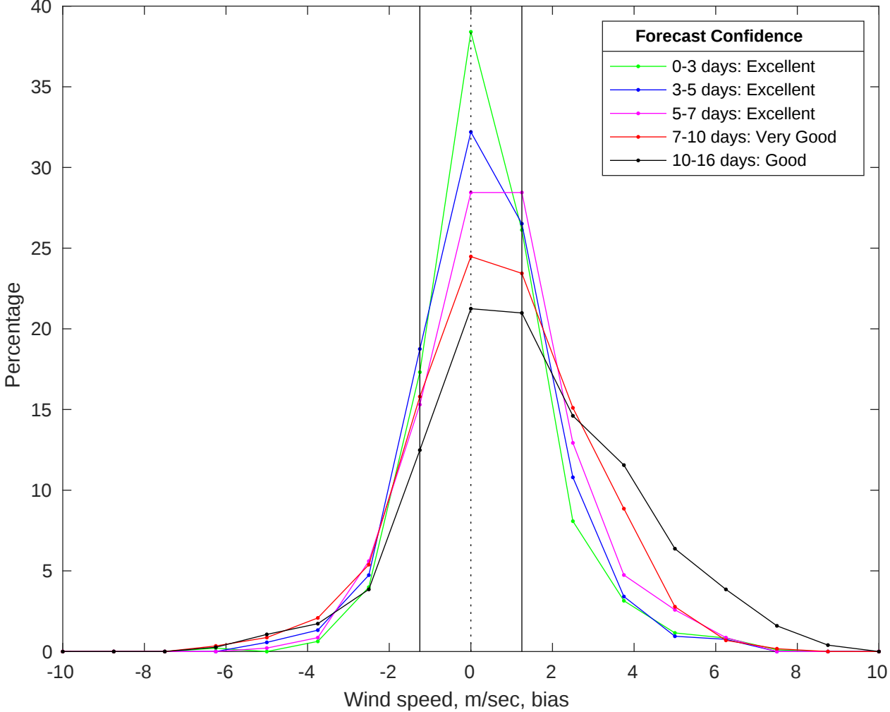
NDBC 42020 vs GFS Winds Bias Histogram: 04-Jul-2025
