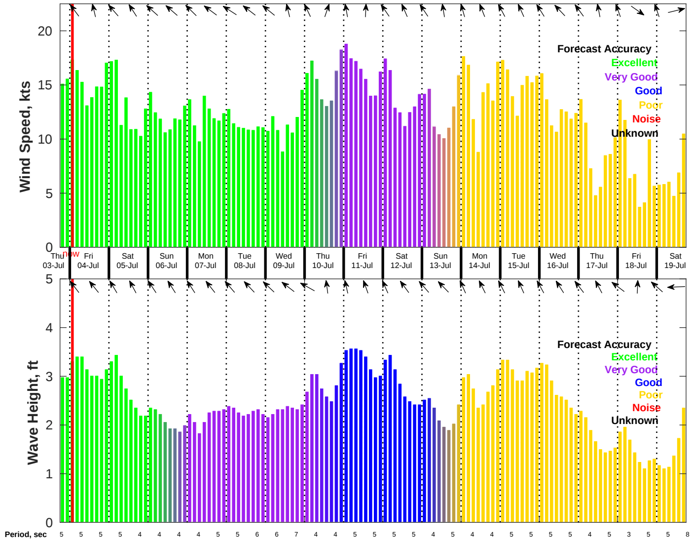
Wind & Wave Forecast for NDBC 42020 from 03-Jul-2025 18:00:00 to 19-Jul-2025 18:00:00
