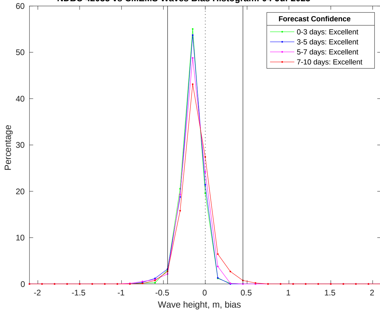
NDBC 42035 vs CMEMS Waves Bias Histogram: 04-Jul-2025
