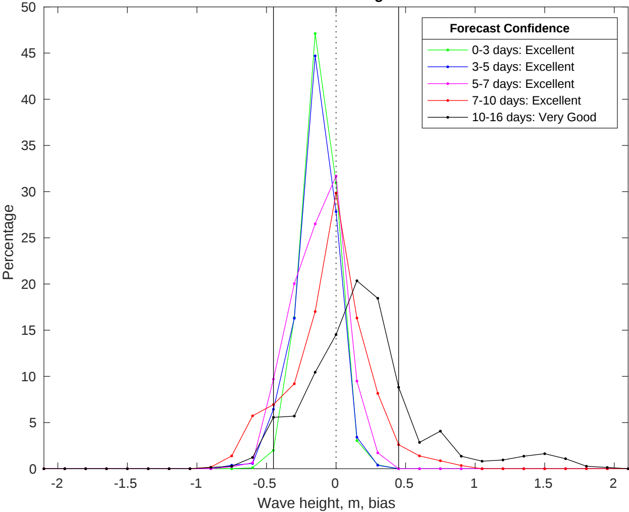
NDBC 42035 vs GFS Waves Bias Histogram: 04-Jul-2025
